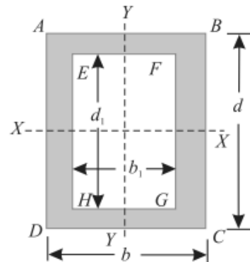
Hollow rectangular section.
